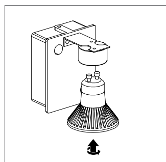
Montage GU10 lamp
