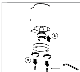
Montage GU10 lamp
