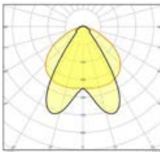
TRUSYS FLEX 50W 4000K 2X30°
