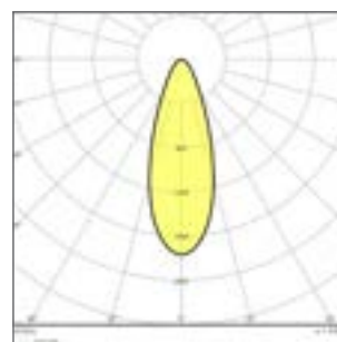
SPOT LED ADJUST 8W 940 PS DIM IP20
