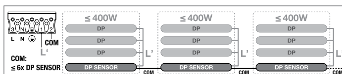
Bedrading leader/follower en leader/leader
